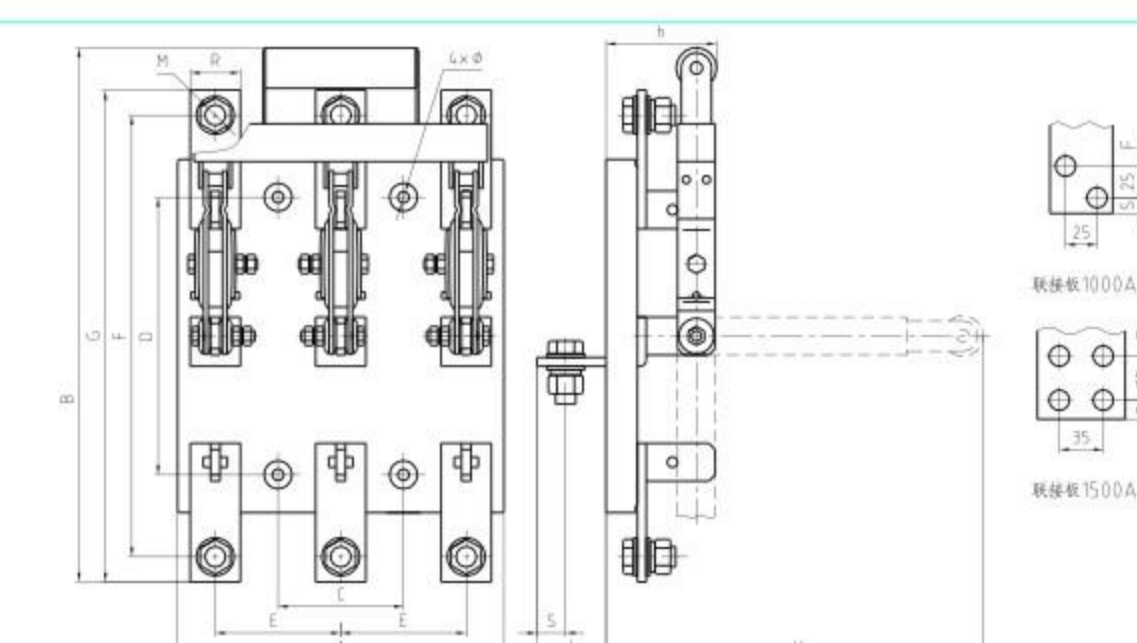
图6 HS11-600~1500(板前接线板后接线)
